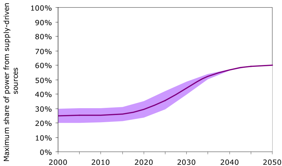
Figure 4 - 8 Constraint placed on PV and wind power due to grid limits. Range represents differences across regions.
